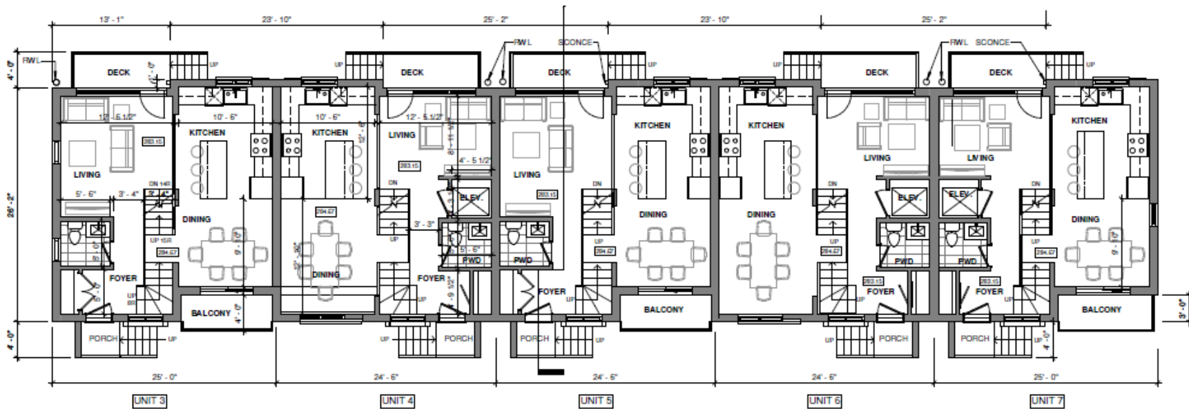
2 GROUND FLOOR PLAN - BLD B 1/8" = 1'-0"
