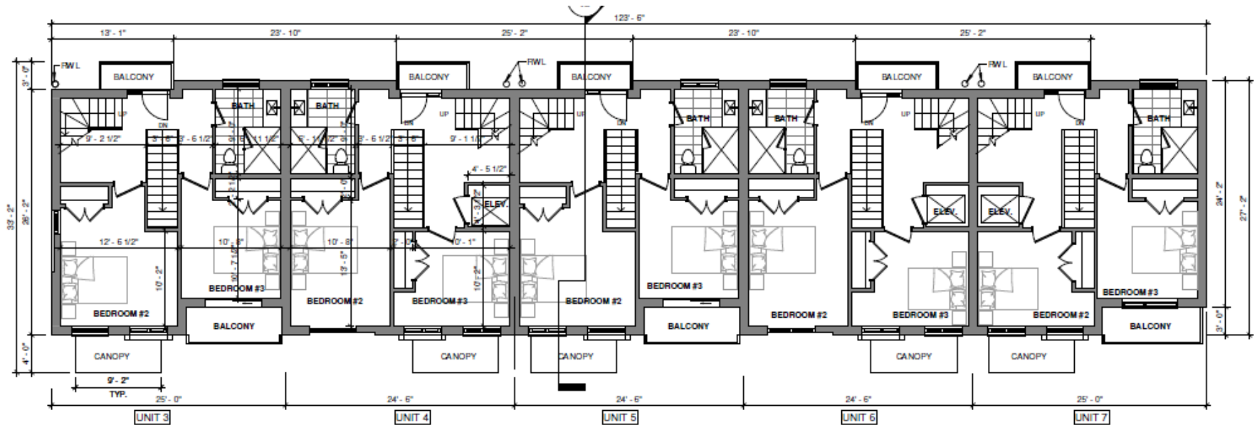
1 SECOND FLOOR PLAN - BLD B 1/8" = 1'-0"
