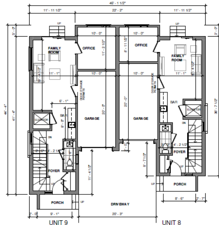
2 1ST FLOOR - SEMI - BLD C 1/8" = 1'-0"
