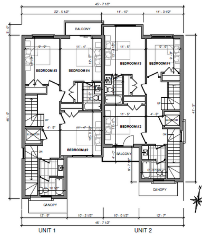
3 2ND FLOOR - SEMI - BLD A 1/8" = 1'-0"
