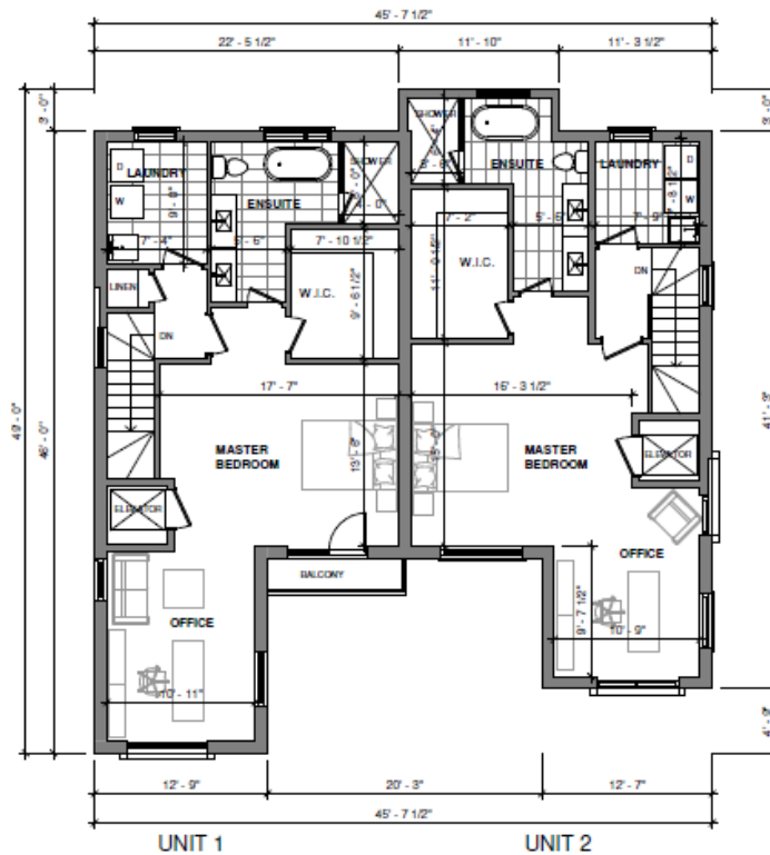
4 3RD FLOOR - SEMI - BLD A 1/8" = 1'-0"
