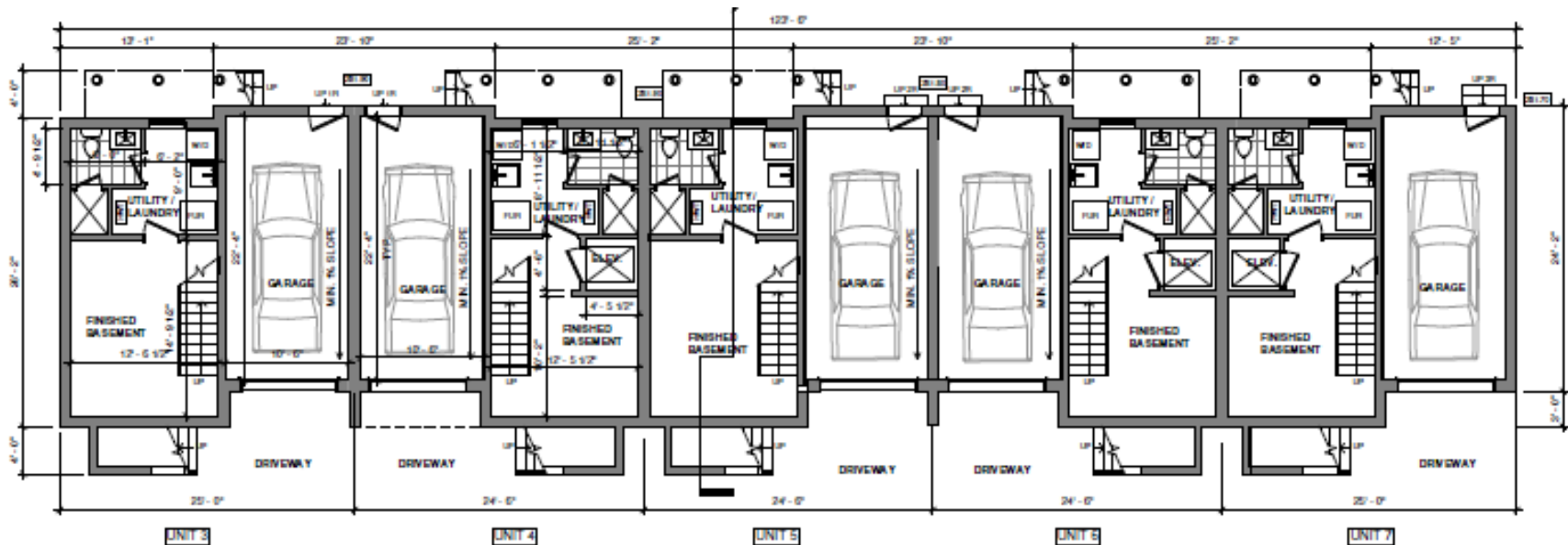
1 BASEMENT PLAN - BLD B 1/8" = 1'-0"
