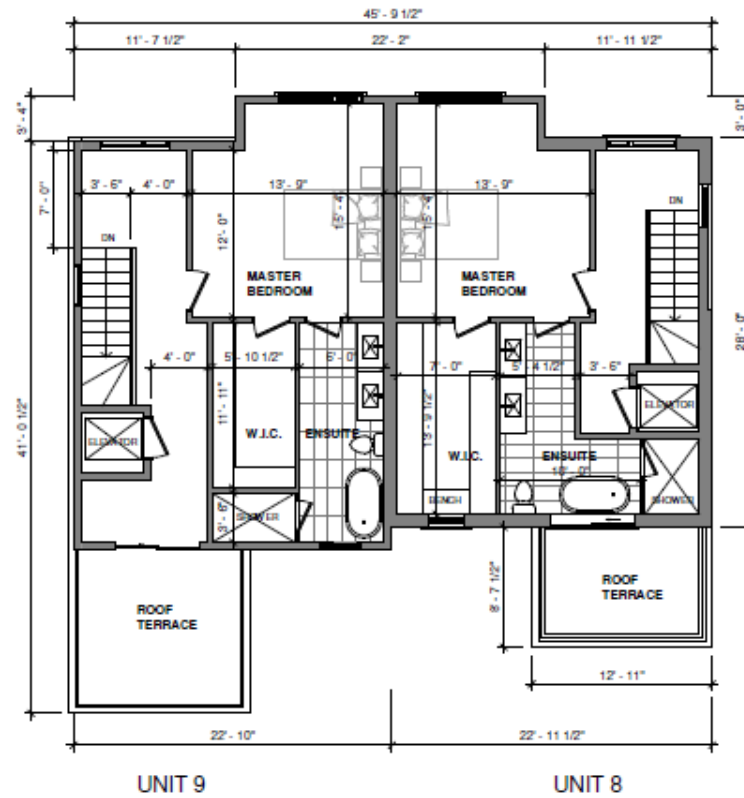
2 4TH FLOOR - SEMI - BLD C 1/8" = 1'-0"
