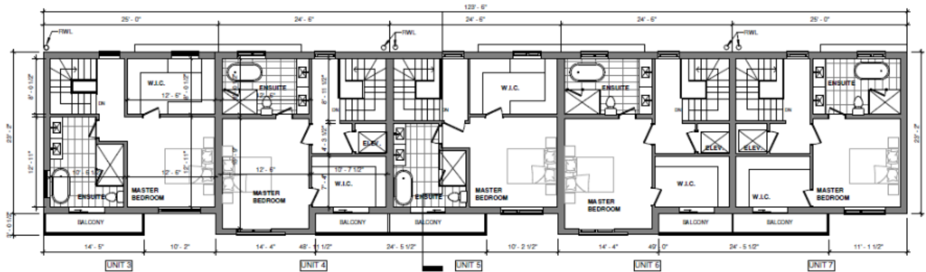
2 THIRD FLOOR PLAN - BLD B 1/8" = 1'-0"
